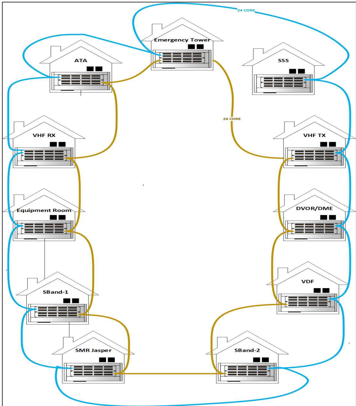
Figure 1: 2x24 Fibre Network Route
